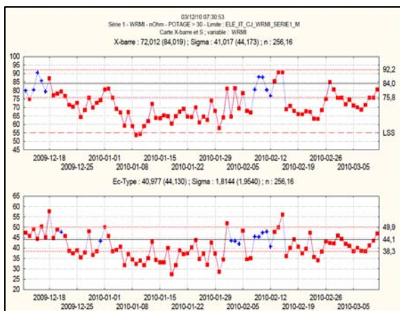
X-bar & S chart of a characteristic related to alumina electrolysis.
